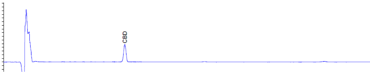
Figure 2. Chromatogram of the analysis
