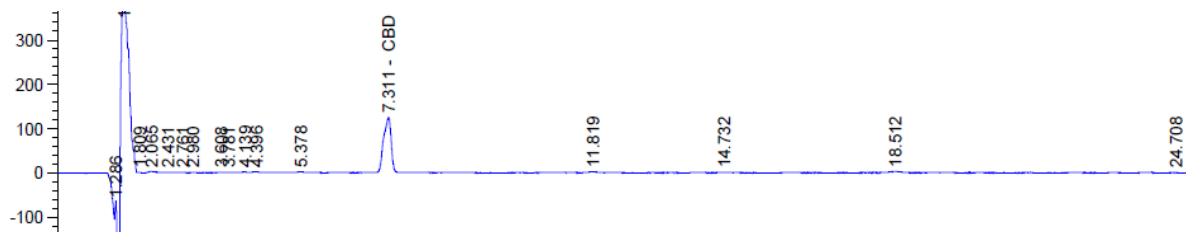
Figure 2. Chromatogram of the analysis
