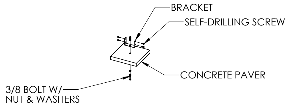
OPTION #2 304 SS ANCHOR BRACKET FOR CONCRETE PAVER STONE. PAVER NOT INCLUDED
