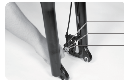
Brake pad Brake caliper 4# L-shaped wrench
