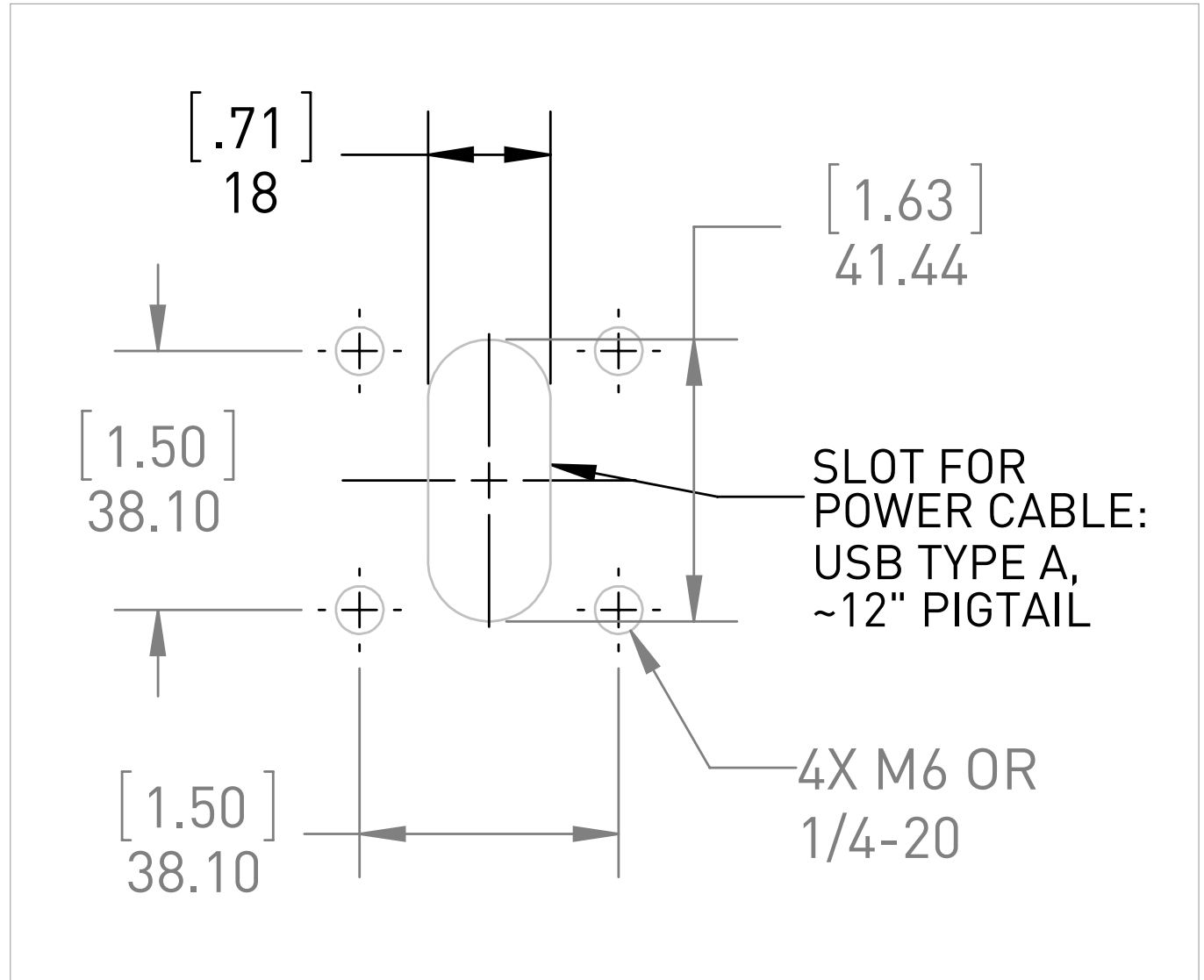
Mounting pattern
