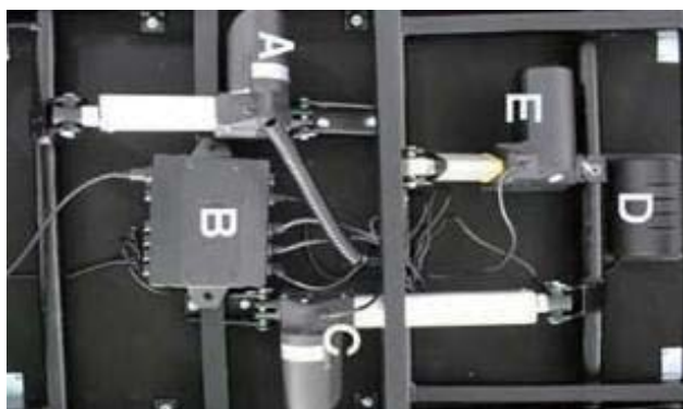
Fig.5.1 Electrical components
