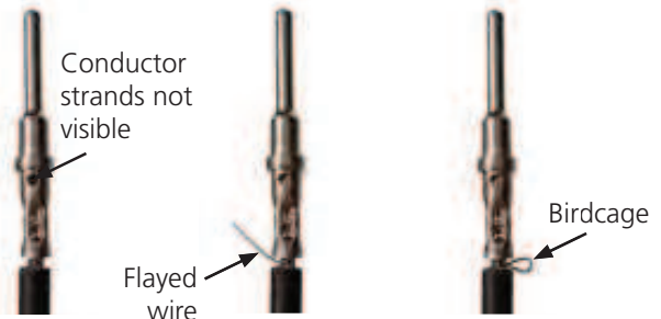
Unacceptable Crimps
