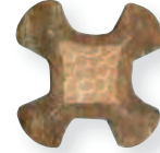
Indenter Crimp Cross-Section Across Axis
