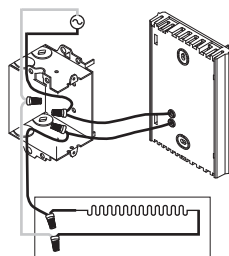
4-wire installation
