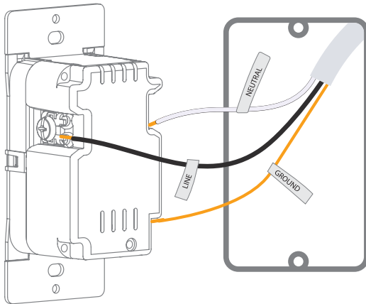
Wiring Diagram
