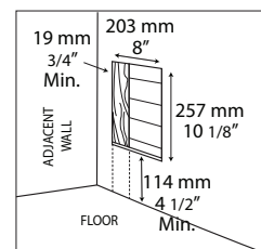
ROUGH-IN: 8" W (203 mm) X 10-1/8" H (257 mm) X 4" D (102 mm)
