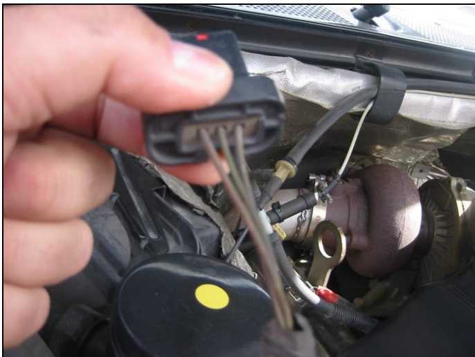
MAP Sensor location 94-97 (Figure 1)
