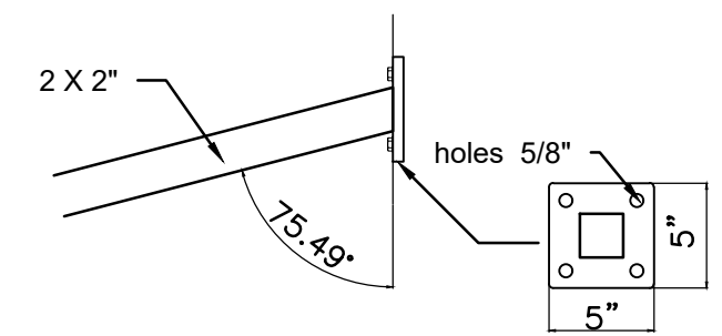
DETAIL 4 - IRON SCALE _____ NONE
