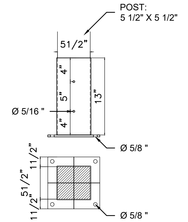
DETAIL 1 - POST BOOT SCALE _____ NONE
