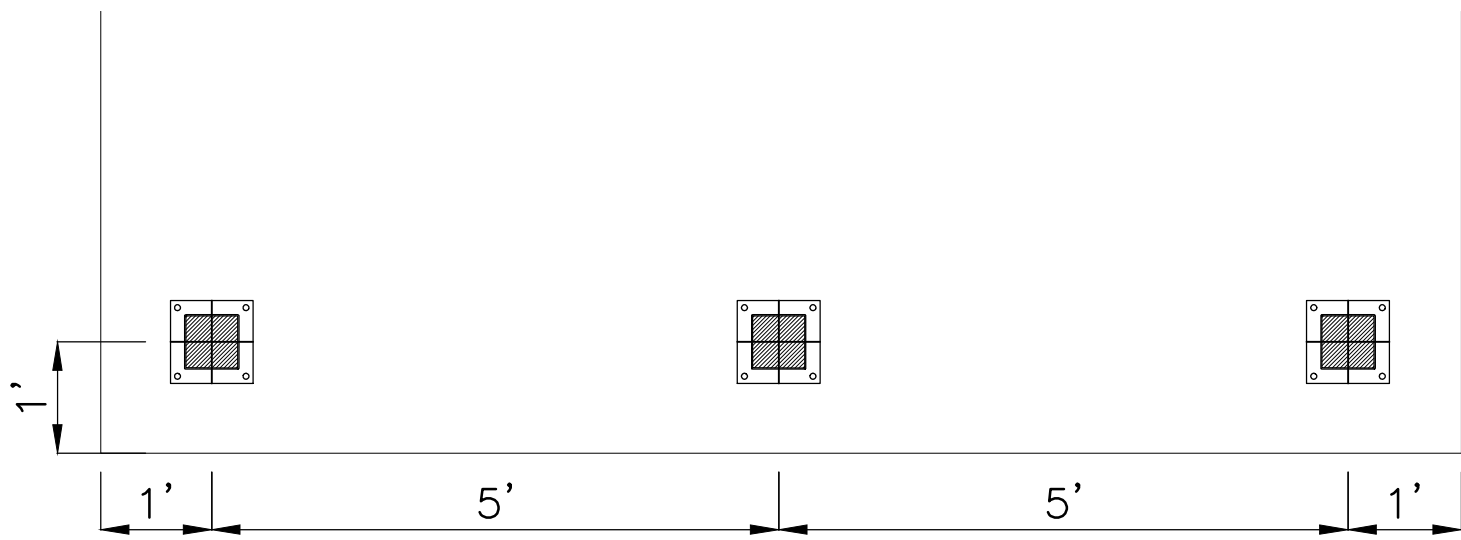
COLUMN LOCATION SCALE _____ NONE
