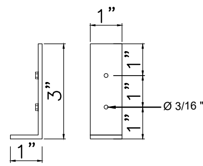
DETAIL 3 - "L" BEAM CONNECTORS SCALE _____ NONE
