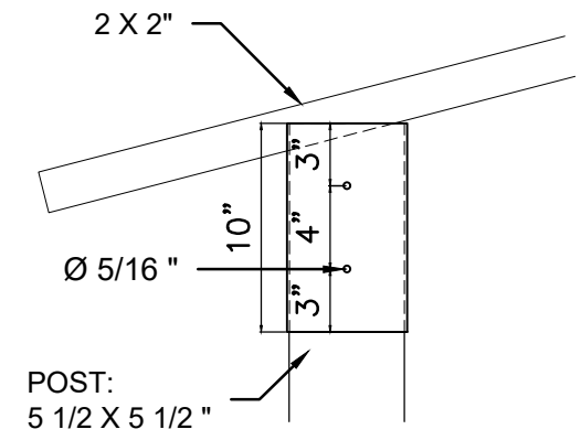
DETAIL 1 - POST BOOT SCALE _____ NONE
