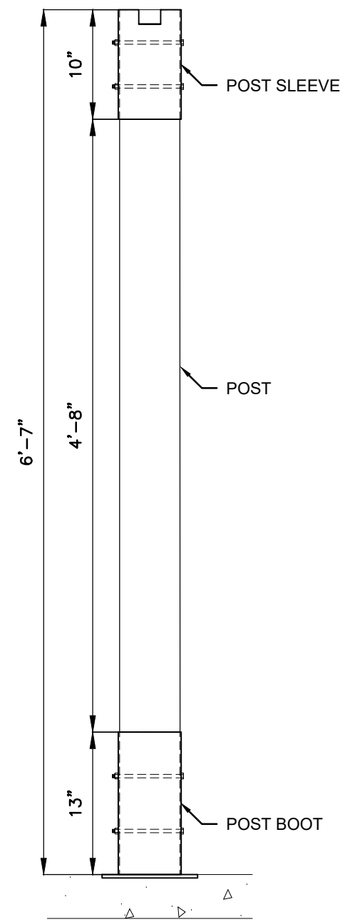
DETAIL - POST SCALE _____ NONE
