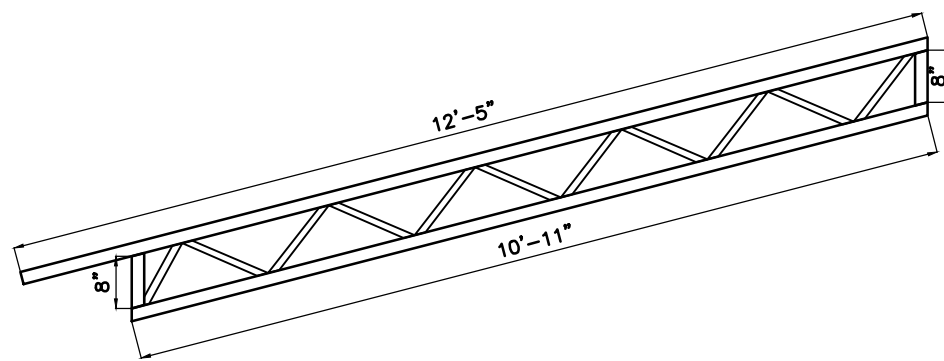
DETAIL - BEAM SCALE _____ NONE
