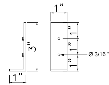
DETAIL 4 - "L" BEAM CONNECTORS SCALE _____ NONE
