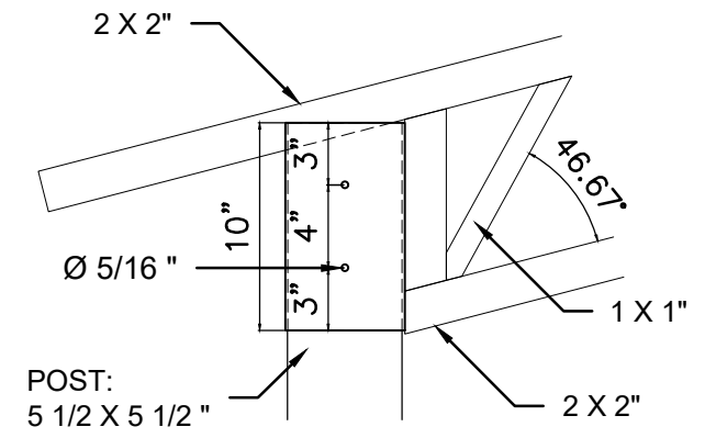
DETAIL 1 - POST BOOT SCALE _____ NONE
