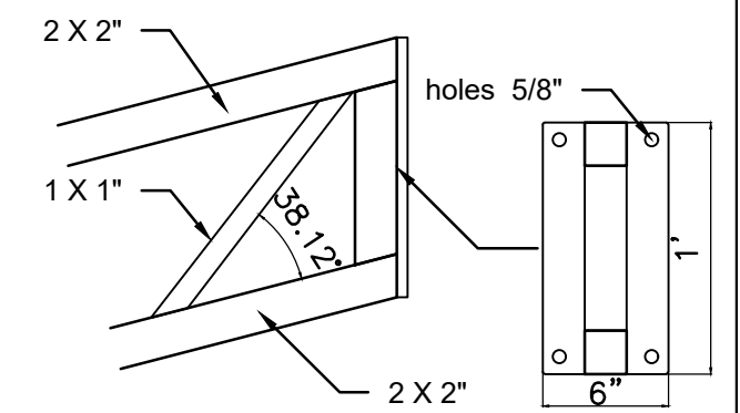
DETAIL 5 - BEAM SCALE _____ NONE
