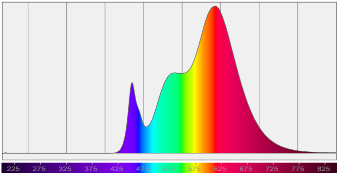
Spectral power distribution (SPD) / W/nm – 0-100%
