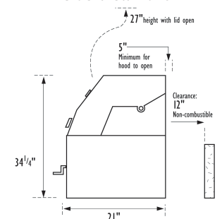
Side View Built In
