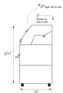
Side View on Cart
