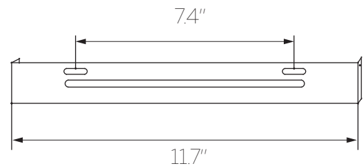
UPPER BRACKET
