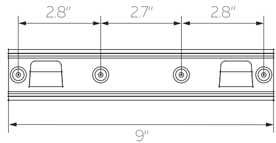
LOWER BRACKET
