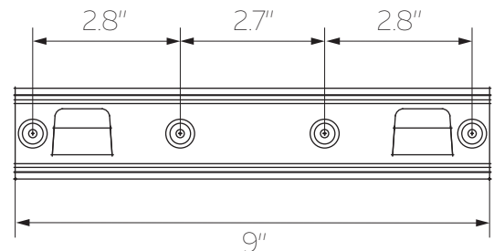
LOWER BRACKET
