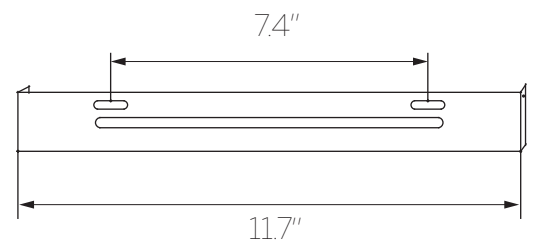
UPPER BRACKET
