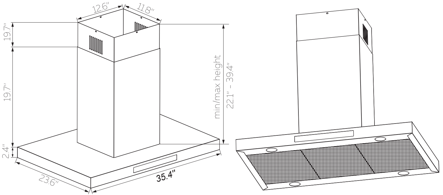
FRONT VIEW
