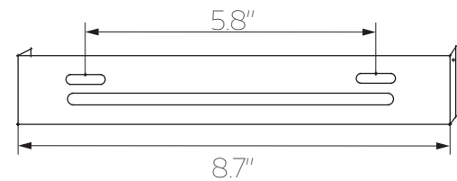
UPPER BRACKET
