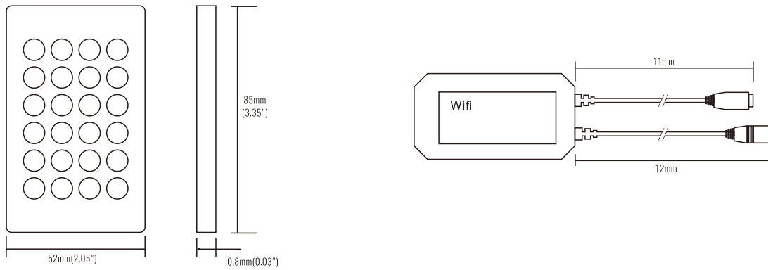
Controller and Receiver
