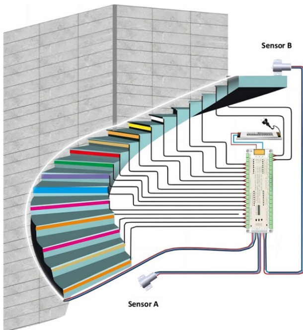
SAMPLE WIRING DIAGRAM
