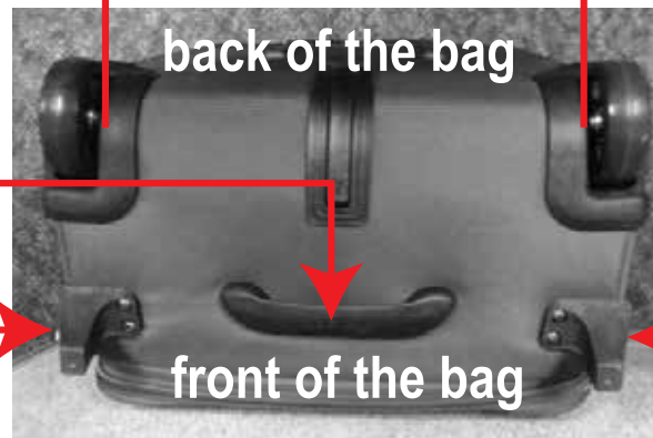
P40712A1142 Wheel axel with (2) ball bearing
