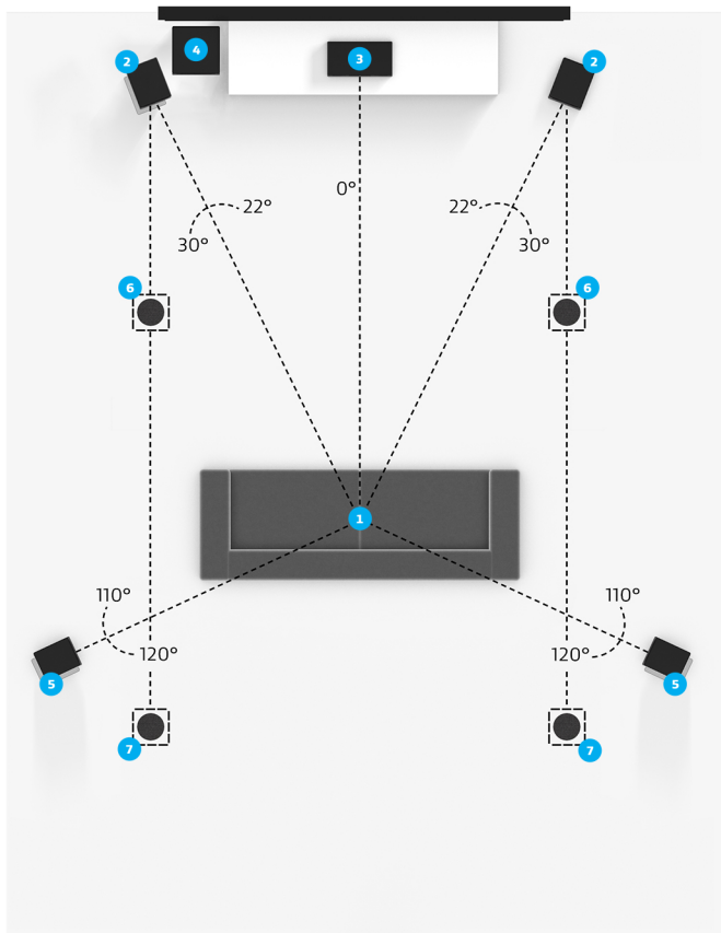
Speaker placement for 5.1.4 setup
