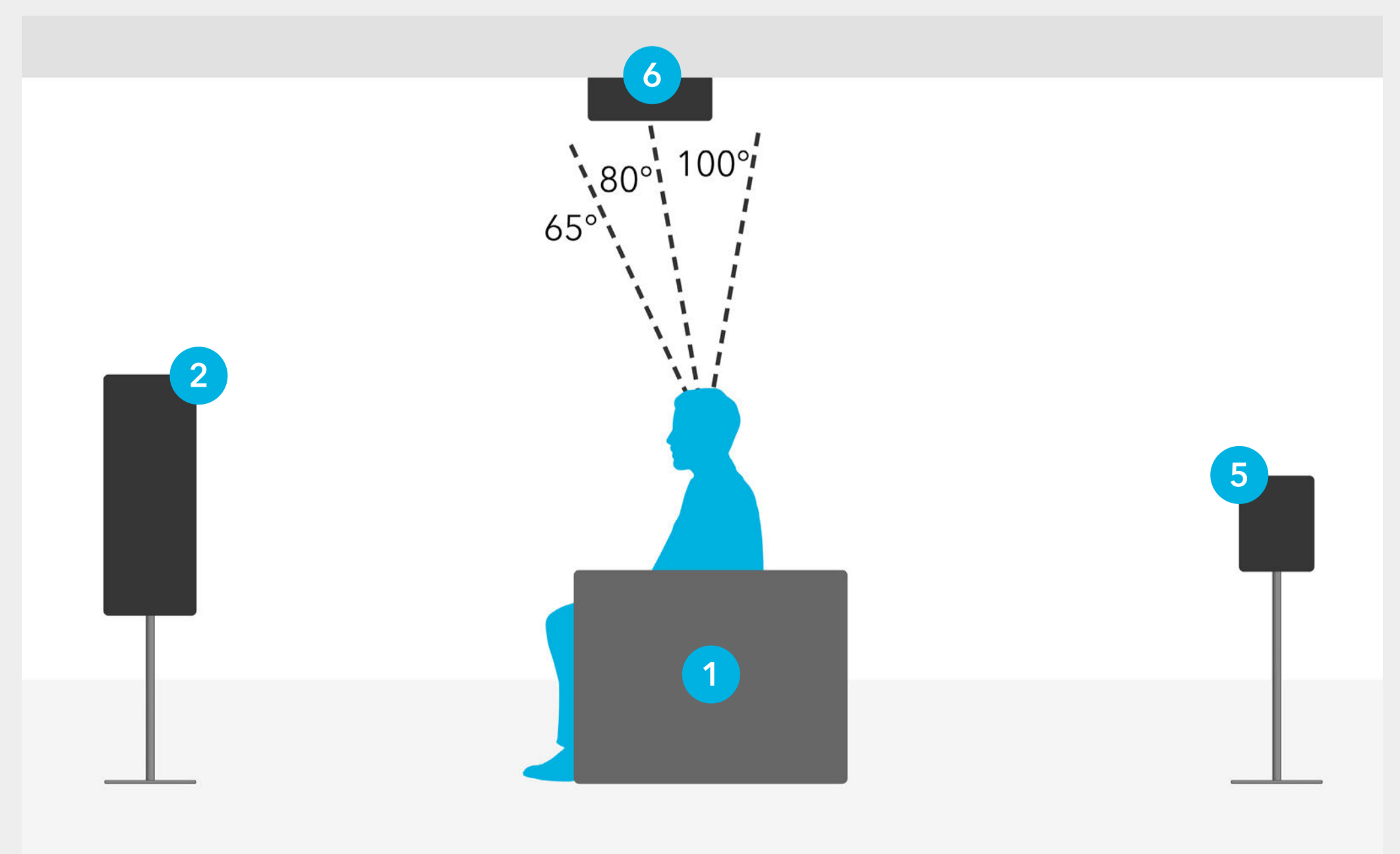
OVERHEAD SPEAKER PLACEMENT DETAIL FOR 5.1.2 SETUP
