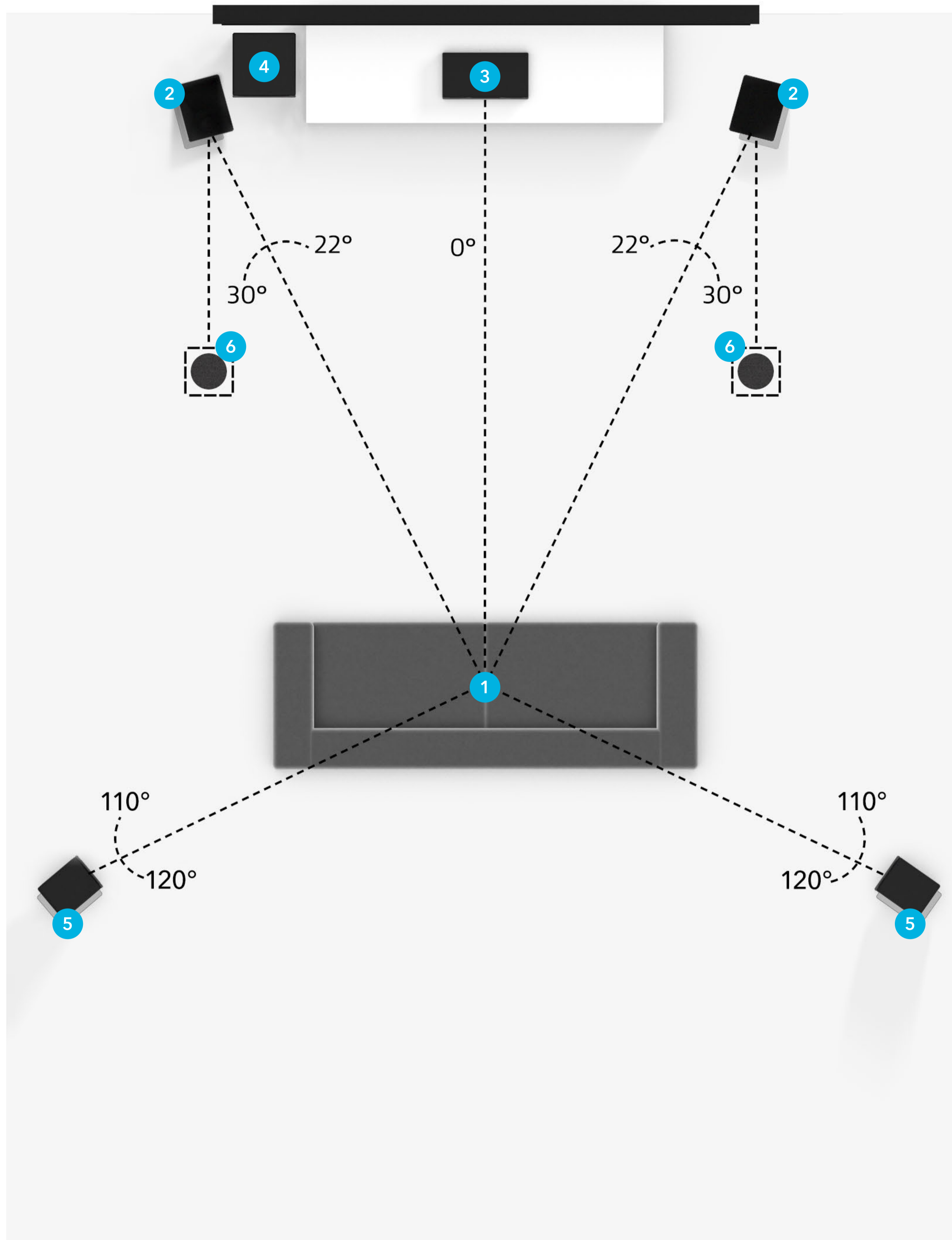
SPEAKER PLACEMENT FOR 5.1.2 SETUP
