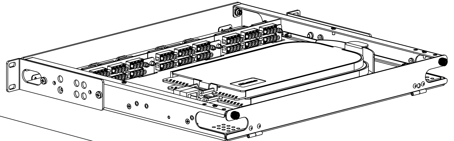
VIEW WITH REAR DOOR OPENINGS TOP PANELS HIDDEN
