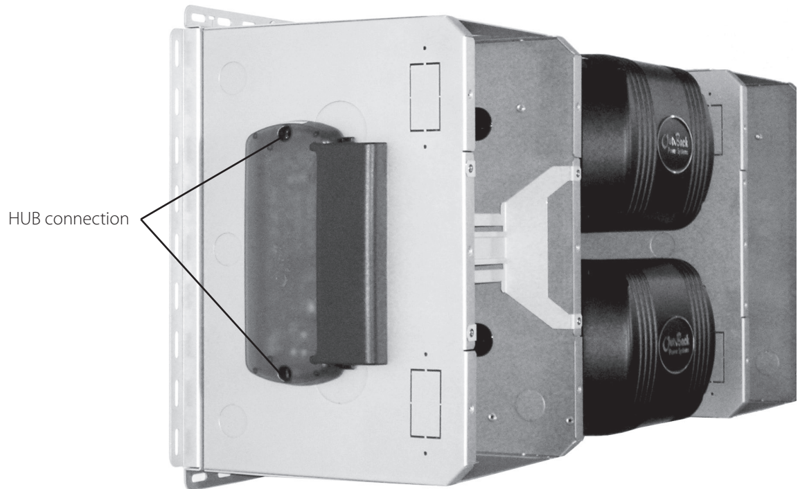
Figure 14: OutBack HUB
