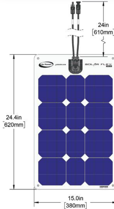
Front Profile
