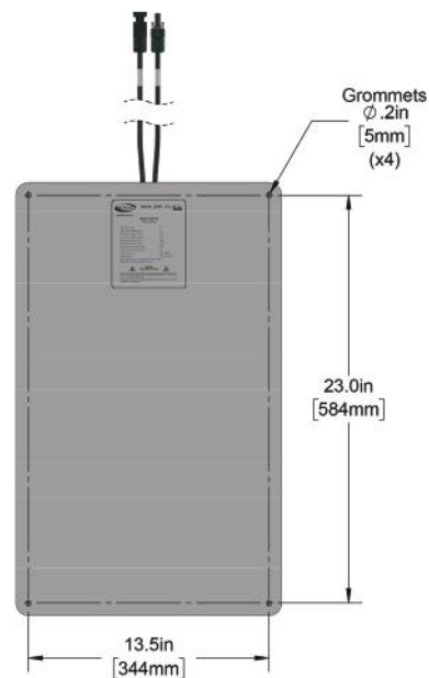
Back Profile
