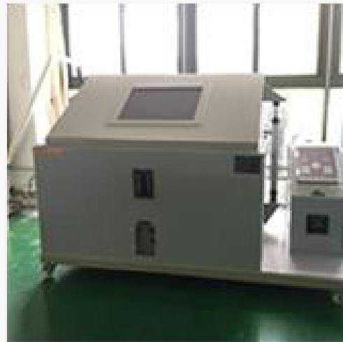
盐雾检测设备 Salt spray detection chamber
