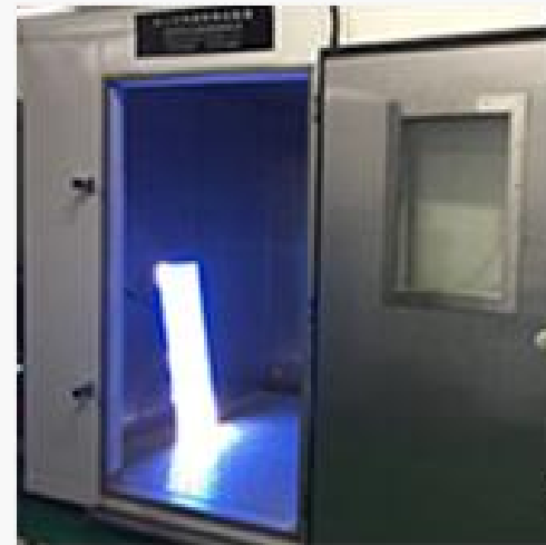
步入式恒温恒湿实验室 Walk-in constant temperature and humidity testing chamber
