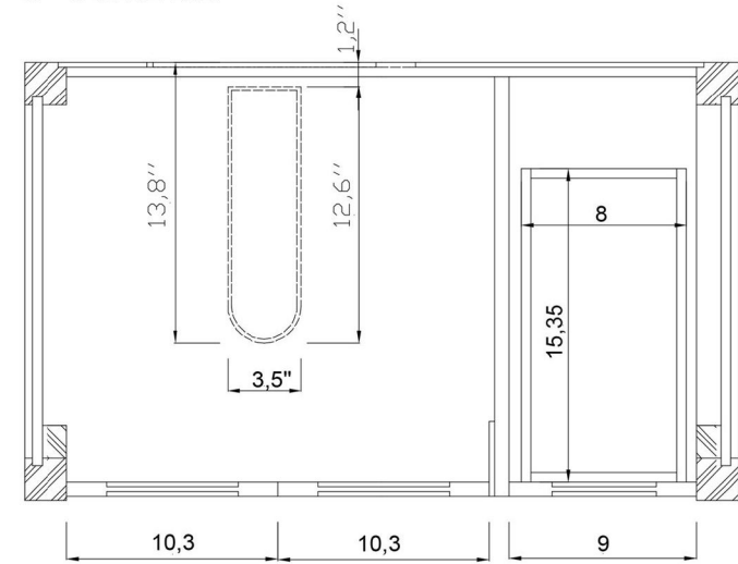
C - C SECTION
