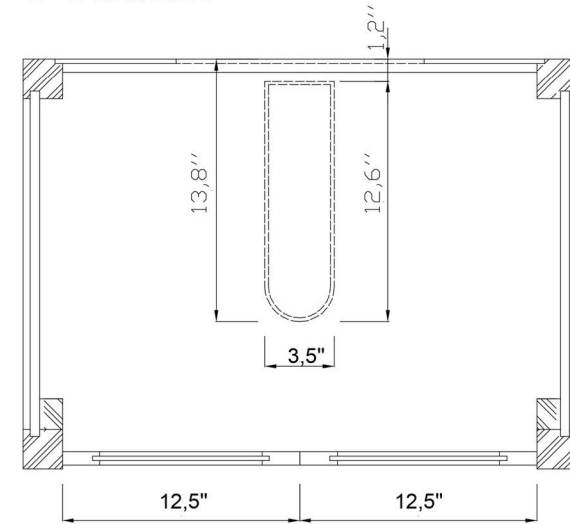
B - B SECTION
