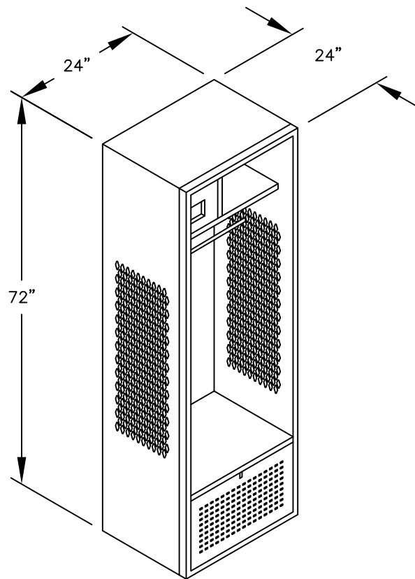
MODEL #70024 OPEN ACCESS STANDARD LOCKER
