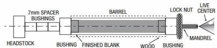
DIAGRAM B – TURNING THE BLANK
