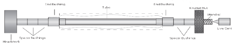
Diagram B - Turning the Blank
