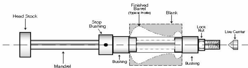
Diagram B / Mounting Parts on the Mandrel
