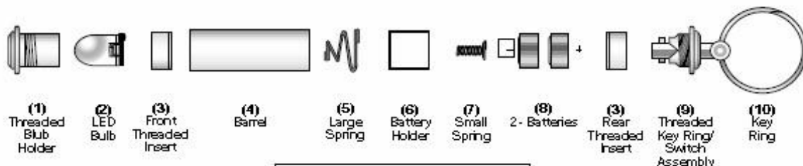
Diagram C / Penlight Assembly
