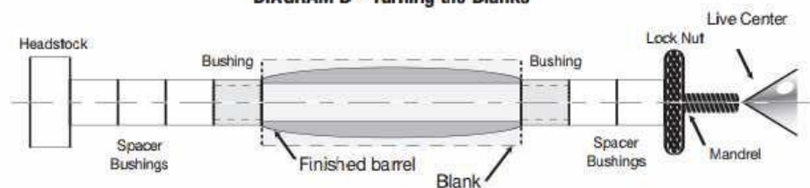
DIAGRAM B • Turning the Blanks
