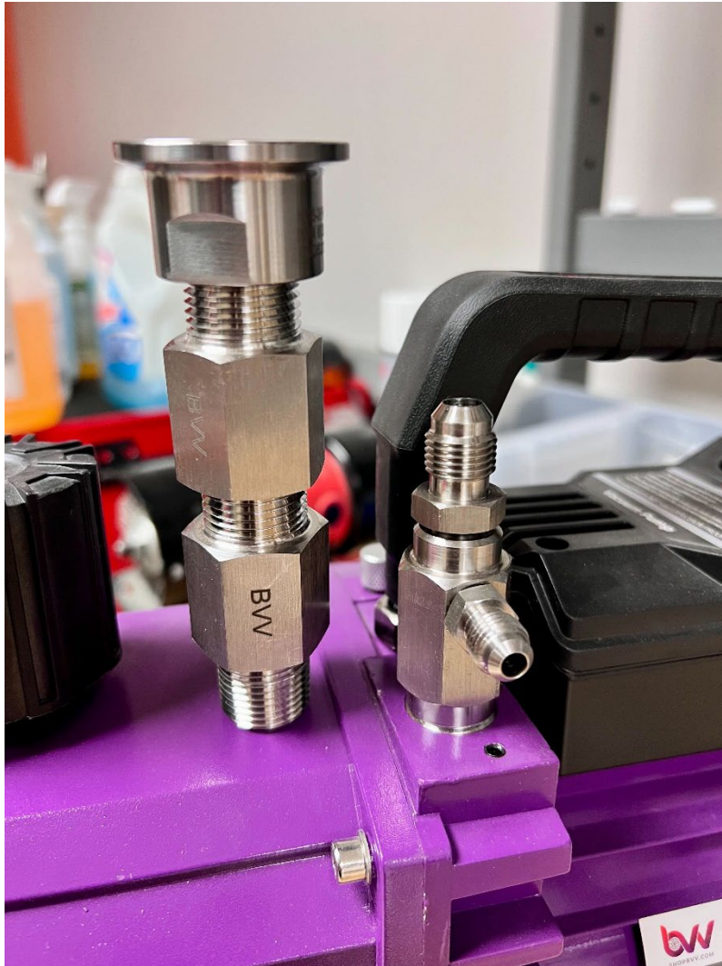
Image 2: KF-25 Extension Next to Tee Fitting
