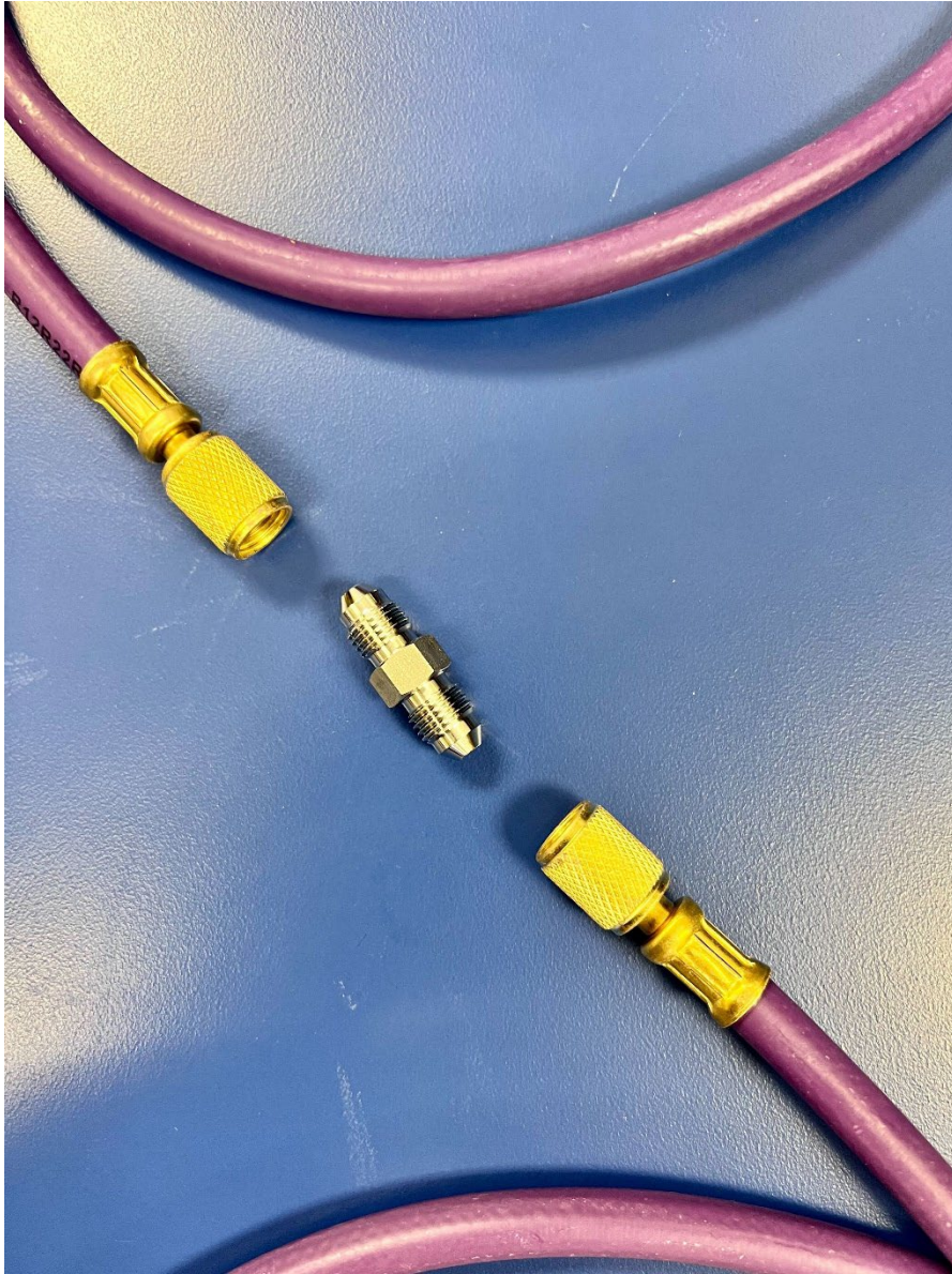
Image 4: 1/4" JIC Union Fitting with Two HVAC Hoses
