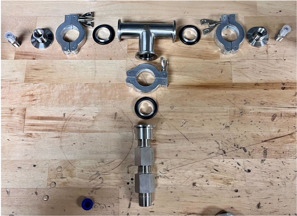
Image A: KF-25 Tee Disassembled
