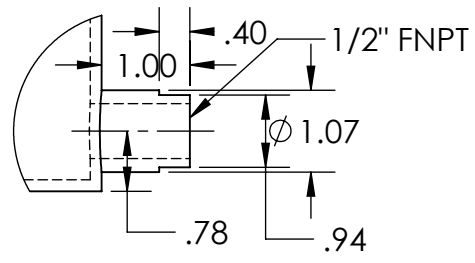
DETAIL P SCALE 2 : 5
