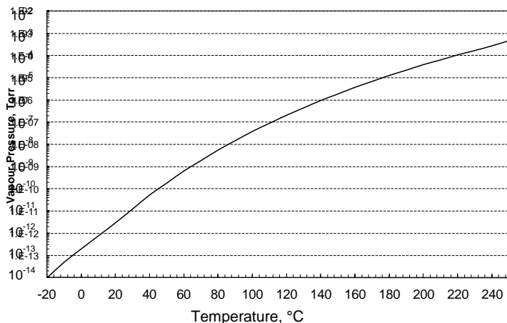
Vapour pressure over working temperature
