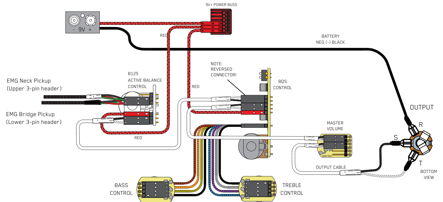
Diagram #3 (preferred wiring order) ABC Control BQS Control Master Volume Output Jack
