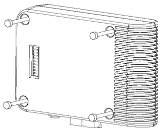
Fig.2 - Wall Mounting
