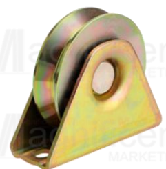
V-Groove Gate Roller #50-Exposed – Php329/pc Roller Size: D50mm Capacity: 100kg
