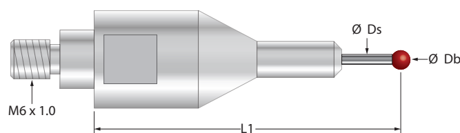
Faro compatible stylus with carbide stem and stainless steel base.
