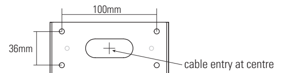
Backplate fixing hole positions:
