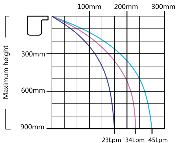
APPROXIMATE PROJECTION OF THE WATER SHEET PER 300MM OF WATERFALL LENGTH
