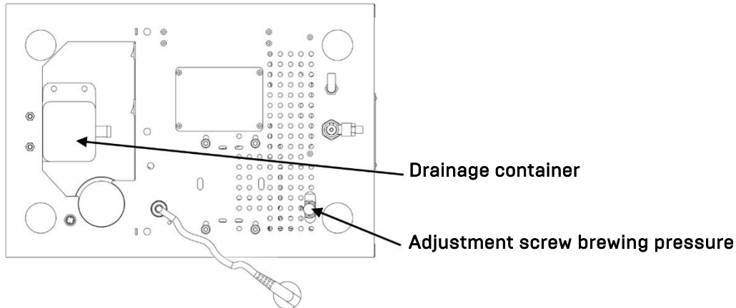
Image 5: Machine bottom
