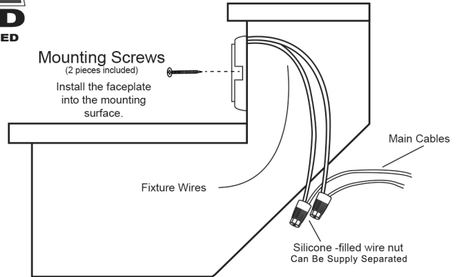
STB07 Sideview of wall mounting
