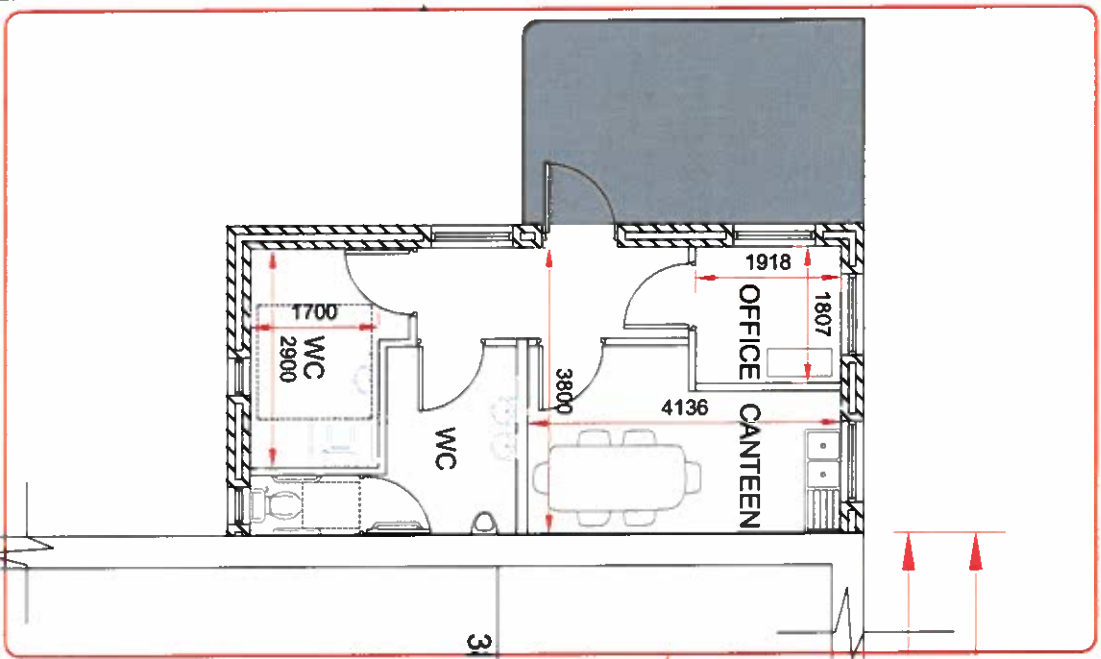
Plan of Admin Building Scale @A1/A3 1:50 / 1:100
