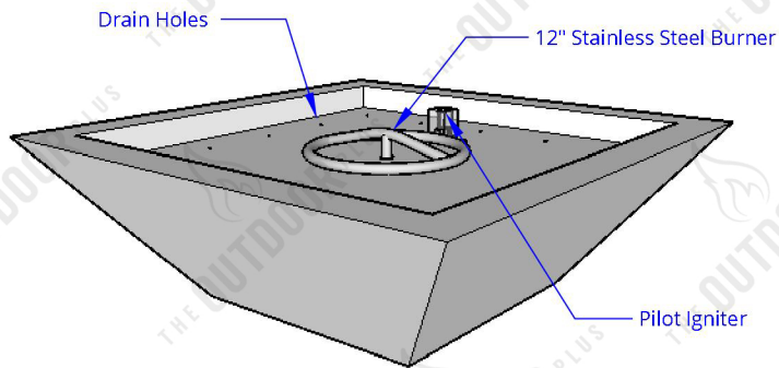
ISOMETRIC VIEW
