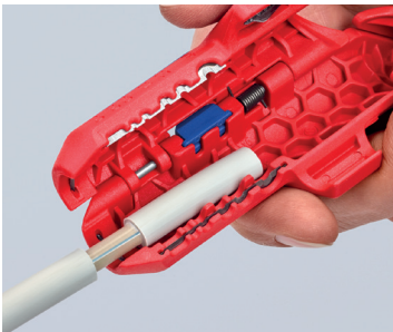
Stripping NYM cable
