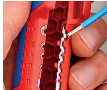
Stripping single conductor wire
