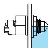
THIN-WALL O-RING & NUT
